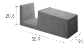
RS 924 Maciza Solid Solide
